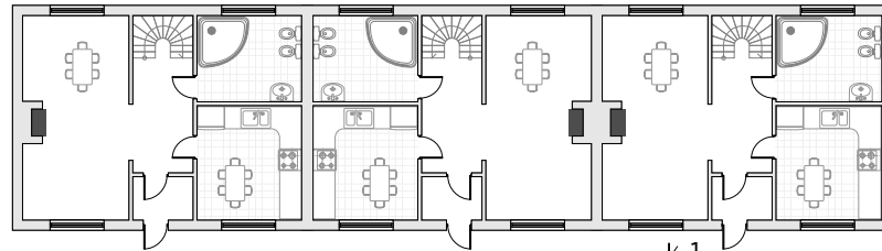
GROUND FLOOR PLAN TOWNHOUSE 3,4,5
