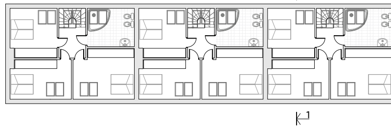
FLOOR PLAN TOWNHOUSE 3,4,5
