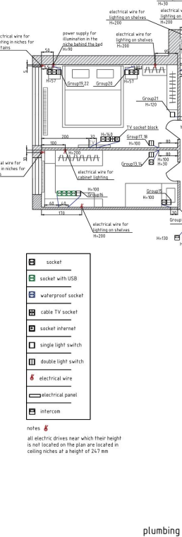
lighting equipment layout plan linked to switches
